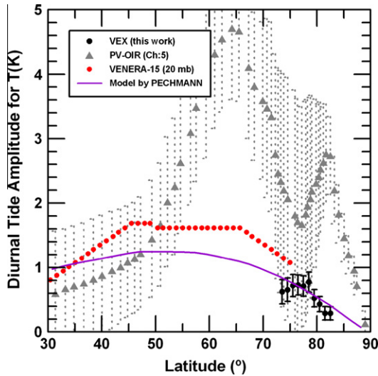
Fig. 10. Meridional structure of the diurnal tide inferred for the temperature. Our results with Venus Express (black circles) are plotted together with Pioneer Venus OIR radio-occultation ( \sim 65 km) measurements (grey triangles, Taylor et al., 1980) and with Venera-15 measurements ( \sim 60 km, red circles, Zasova et al., 2007). The purple line displays the Pechmann and Ingersoll (1984) tidal model results ( \sim 65 km). (For interpretation of the references to colour in this figure legend, the reader is referred to the web version of this article.)
