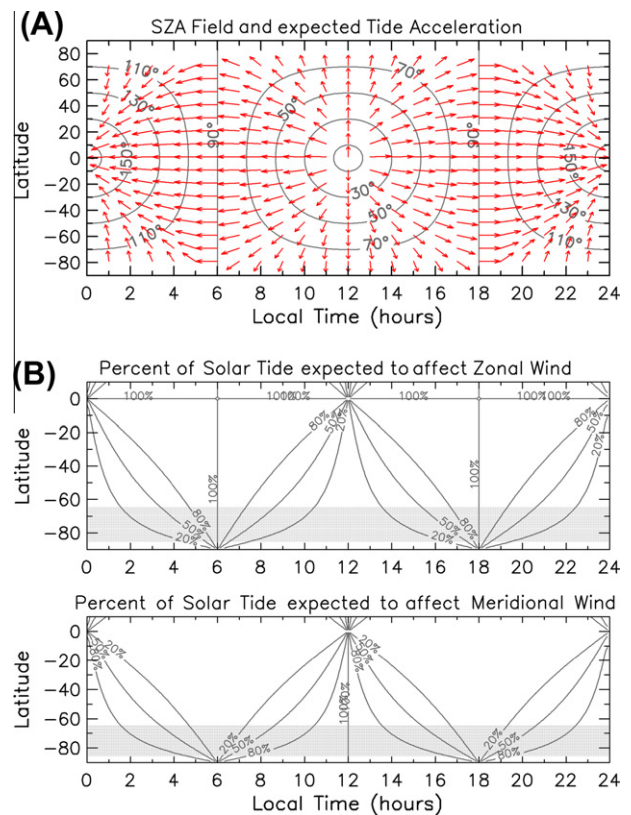
Fig. 9. The latitude vs. solar local time map of the expected solar-to-antisolar flux for the diurnal tide (panel A) and percentages of tidal contribution on the zonal and meridional component of the wind (panel B). The wave fronts are assumed to be tangent to the lines of constant solar zenith angle (line contours) while the red arrows indicate both negative pressure gradients and the sense of the tidal wind acceleration (panel A). The percentage of total tidal contribution affecting each component of the wind is shown in panel B with contour lines and the region of our study shaded in grey. (For interpretation of the references to colour in this figure legend, the reader is referred to the web version of this article.)
