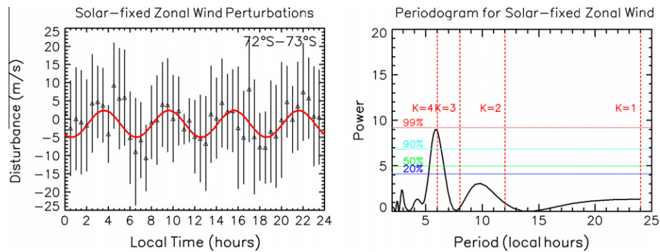
Fig. 5. Average of solar-fixed zonal wind disturbances (left) and their corresponding periodograms (right) for the latitude bin 72°S–73°S. The best sine fit is displayed with a continuous line in the wind disturbances on the left panel. Confidence levels (horizontal dotted lines) and the main solar tide harmonics (vertical dashed lines) are also marked in the periodogram on the right.
