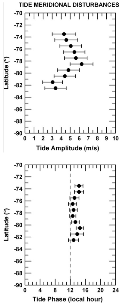
Fig. 7. Latitudinal behaviour for the diurnal tide's amplitude and phase in the meridional wind, in the range 70–85°S. The top panel displays the tidal amplitude and the bottom one the tidal phase. The phase has been defined as the position of the highest tidal acceleration in the poleward sense. Noon is marked with a grey dashed line.
