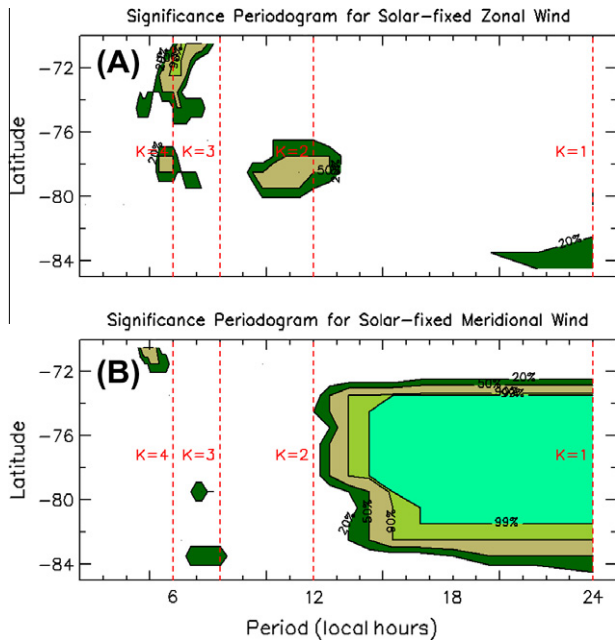
Fig. 3. Significance maps for Lomb-Scargle periodograms inferred from zonal (panel A) and meridional (panel B) solar-fixed wind disturbances in the latitude interval 70–85°S. The data were averaged in latitude bins of 1°. The main solar tide harmonics are marked with dashed vertical lines.
