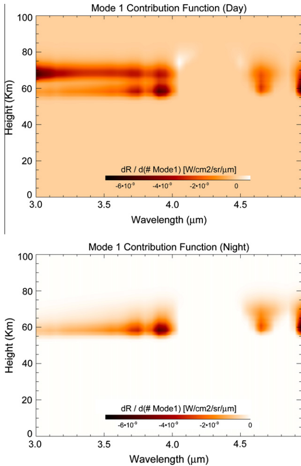
Fig. 2. The Venus mode1 (haze) contribution function from 3.0 to 5.0 \mu\text{m} , with the dayside in the upper panel and nightside in the lower one. Units are described as the amount of radiance change per unit change of particle density. The nightside emissions from 3.9 and 5.0 \mu\text{m} probe the same altitude, centred at about 60 km. The lack of emission between 4.0 and 4.5 \mu\text{m} is due to strong \text{CO}_2 absorption at these wavelengths. For the dayside thermal emission, the contribution function at 5.0 \mu\text{m} is similar to the nightside emission, but the 3.9 \mu\text{m} emission is distinctly different, owing to the more effective scattering of small haze particles at the cloud tops at shorter wavelengths.
