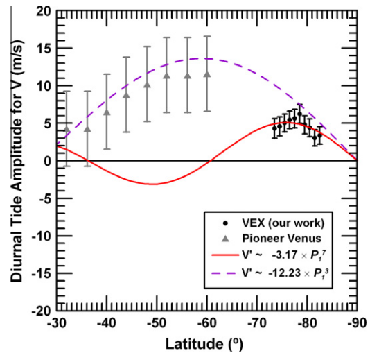
Fig. 8. Meridional structure for the amplitude of the diurnal tide affecting the meridional component of the wind. Our results are plotted with black circles, while the grey triangles correspond to cloud tracking results from UV images with the Pioneer Venus OCPP instrument (Limaye, 2007). Best fits to Legendre polynomials are also shown, with a continuous red line for Venus Express and dashed purple line for Pioneer Venus. A meridional wavenumber 2 is obtained for Pioneer Venus winds, while 6 is the best fit for our results. Numerical values are indicated in the legend.
