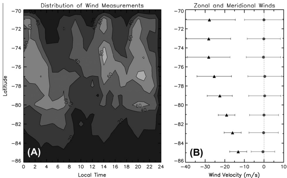
Fig. 1. Distribution of wind measurements with latitude and local time (panel A) and the corresponding zonally averaged profiles for the zonal (triangles) and meridional (circles) components of the wind (panel B). Both panels show post-filtering measurements.
