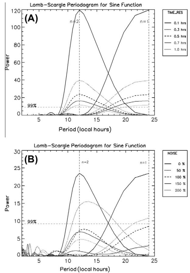
Fig. 4. Lomb-Scargle periodograms for synthetic sinusoidal functions with wavenumbers 1 and 2, for different sampling/local-time resolutions (panel A) and added noise (panel B). The confidence level of 99% is also marked. Harmonics 1 and 2 are marked with dashed vertical lines.
