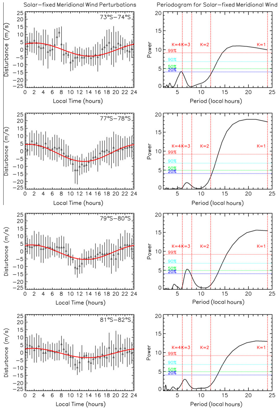
Fig. 6. Same as Fig. 5, for the averages of solar-fixed meridional wind disturbances (left column) and their corresponding periodograms (right column) for several latitude bins.
