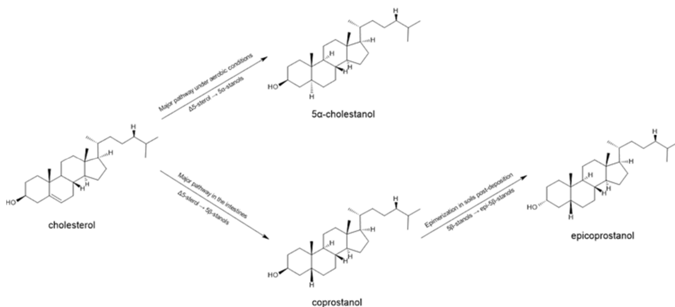
Figure 7. Simplified schematic of the biochemical pathway of the \Delta^5 -sterol (cholesterol) reduction to 5\alpha -stanols and 5\beta -stanols in the natural environment and inside the gut (according to Bull et al. 2002 [43], Sistiaga et al. 2014 [24], Prost et al. 2017 [34]).
