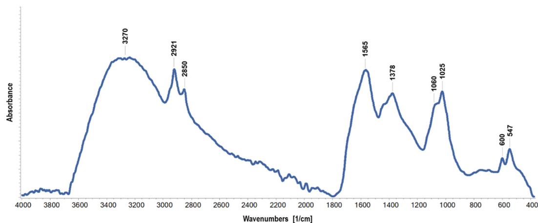
Figure 3. ATR-FT-IR spectra (4000–400 \text{cm}^{-1} ) of an archaeological sample from the cylindrical vessel.
