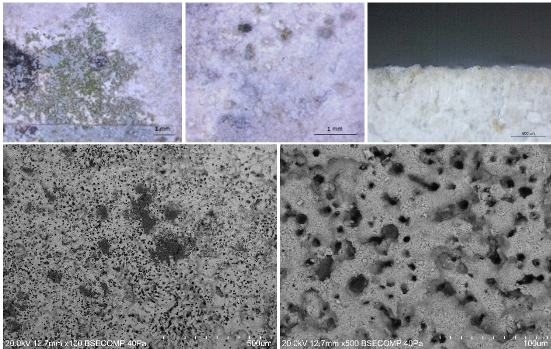
Figure 5.7. Optical microscopy and SEM image of the fs-UV laser cleaned sample surface.
