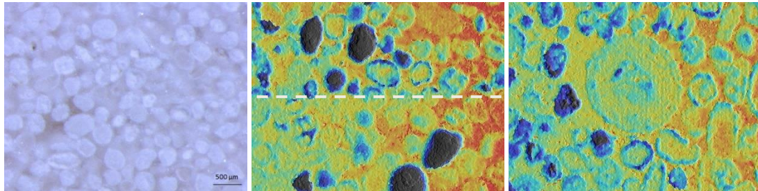
CDR3 ZONE II cleaned by ps-UV laser (optical, confocal edge, confocal inside)
