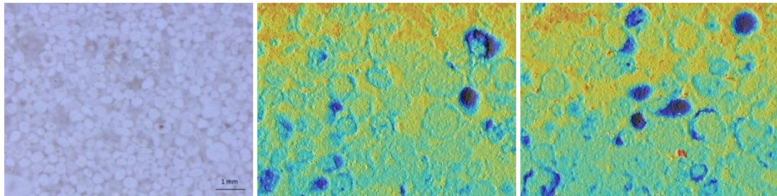
CDR4 ZONE III cleaned by ps-IR laser (optical, confocal edge, confocal inside)
