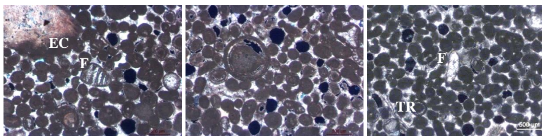
Limestone from Batalha Monastery, royal cloister west gallery (G=Gastropod, GA=Gymnocodiacean algae, B=Bivalve, BR= Brachiopod, F=Foraminifera (miliolid), IN=Intraclast)
