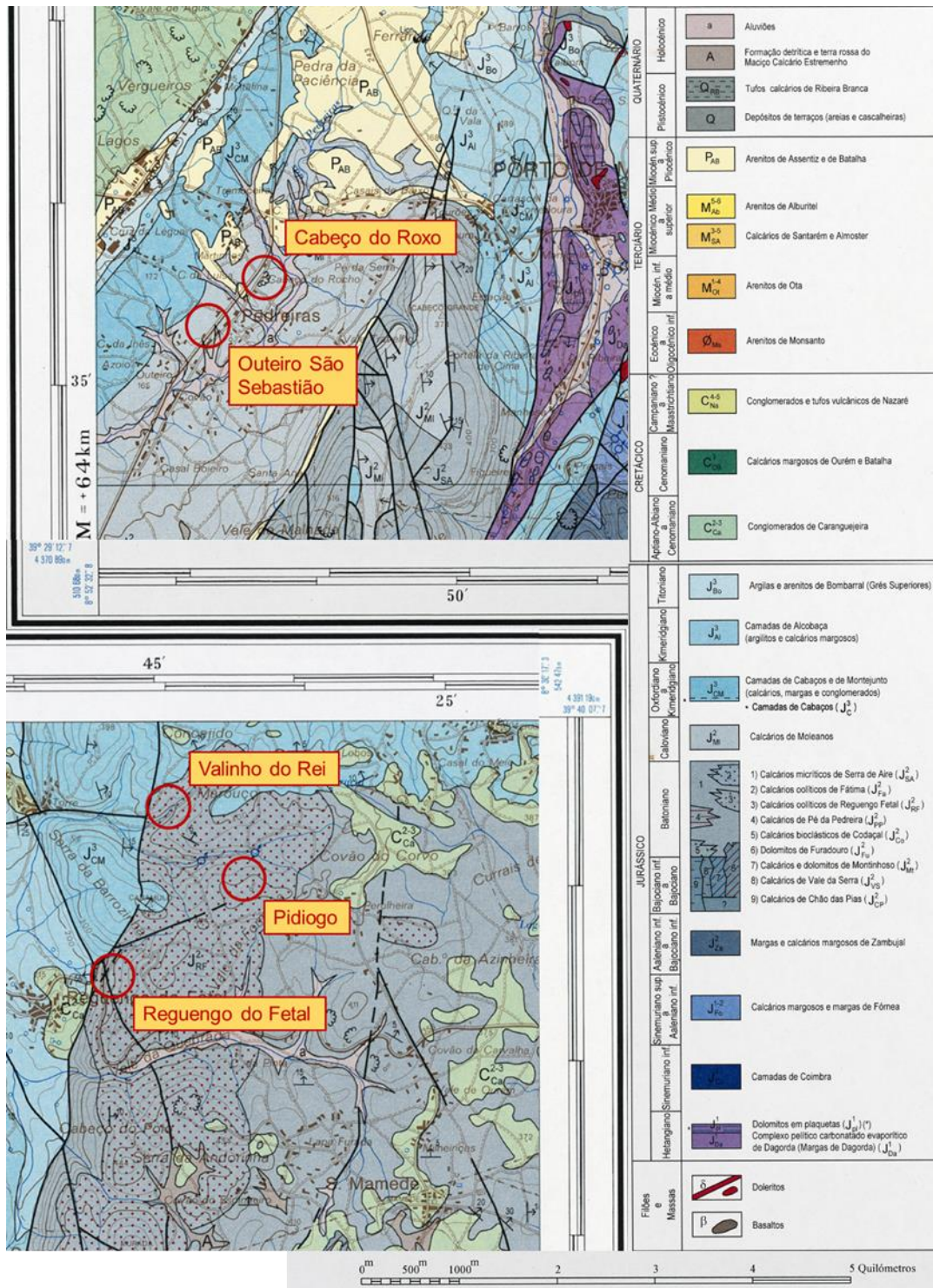
Figure 1.6. Quarries marked on the Carta Geologica de Portugal and their geological settings [25].
