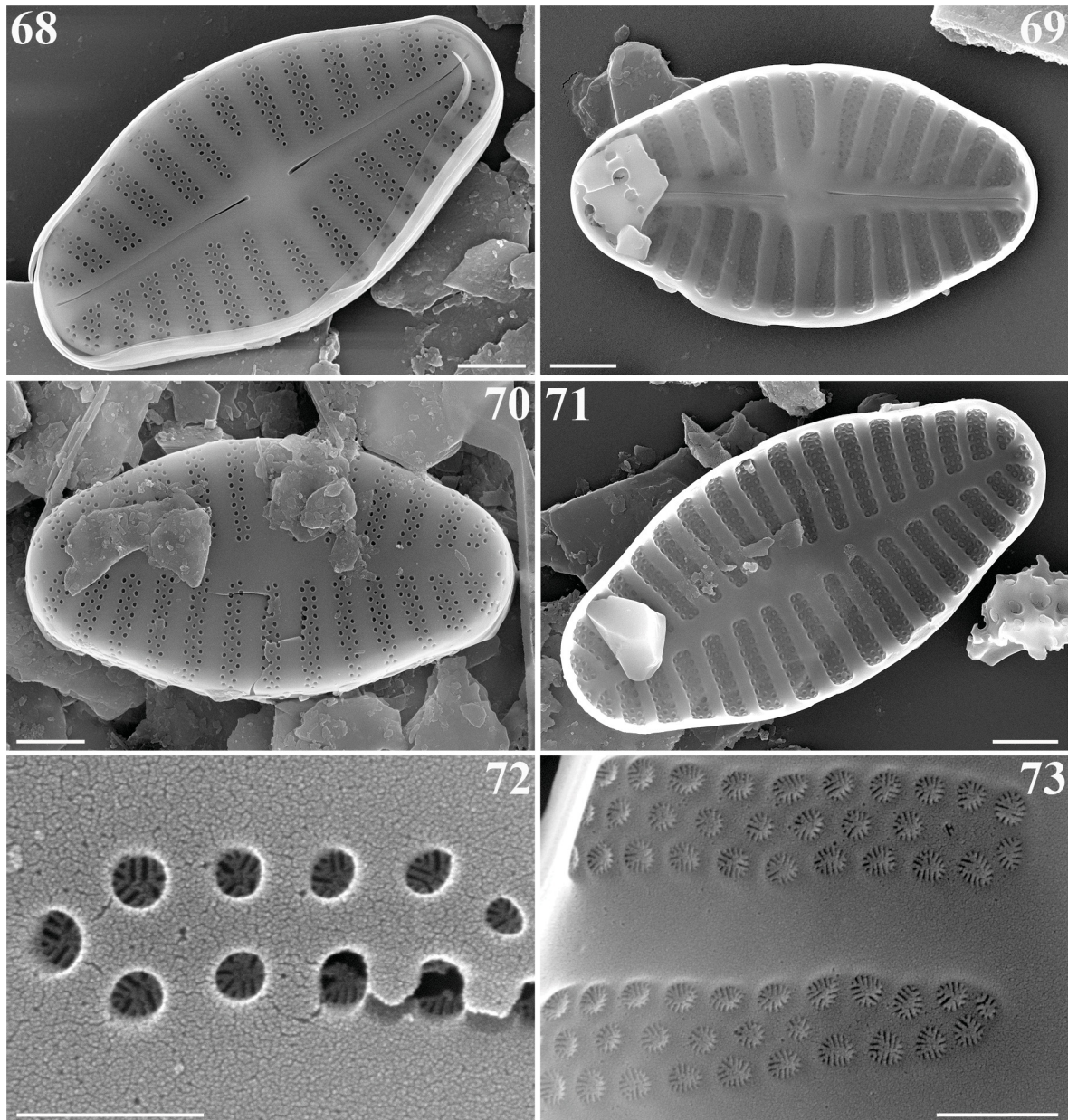
FIGURES 68–73. SEM images of Planothidium audax sp. nov. from type material BR-4663, Limas Stream, Portugal (68, 70–73) and Maria Delgada Stream (69). 68. External view of RV. Notice slightly deflected terminal raphe ends in the same direction and opposite proximal raphe ends. 69. Internal view of RV showing central and polar nodules. Notice slightly deflected proximal raphe ends. 70. External view of SV. 71. Internal view of SV. 72. Close up on striae as seen in external view on SV showing hyemate occlusions of the areolae. 73. Close up on striae as seen in internal view on SV showing hyemate occlusions. Scale bar: 0.25 \mu\text{m} (Fig. 72), 0.5 \mu\text{m} (Fig. 73), 1 \mu\text{m} (Figs 68–71).
