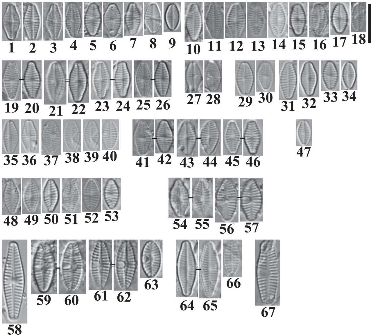
FIGURES 1–67. LM images of Planothidium spp. from two temporary streams in southern Portugal. 1–26. P. audax sp. nov. from type material BR-4663, Limas Stream, Portugal, pool collected on 20 th September 2017 (Figures 1–9 RV, 10–18 SV, 19–26 paired valves of 4 individuals are shown, 21–22 correspond to the holotype). 27–28. RV and SV of two different specimens from Limas Stream, Portugal, dry biofilm collected on 19 th February 2018. 29–34. Specimens from Limas Stream, Portugal, pool collected on 6 th June 2018 (Figures 29–30 RV, 31–34 SV). 35–40. Valves from Limas Stream, Portugal, pool collected on 27 th July 2018 (Figures 35–36 RV, 37–40 SV). 41–46. Population found in Maria Delgada Stream, Portugal, pool collected on 19 th September 2017 (paired valves of three different specimens are presented). 47. Single RV valve found in Maria Delgada Stream, Portugal, pool collected on 28 th May 2018 and representing the smallest valve found for the new species. 48–67. Other Planothidium species found in type material BR-4663, Limas Stream, Portugal (48–53 P. minutissimum , 54–57 paired valves of two specimens of P. rostratoholarcticum , 58–63 P. victorii , including paired valves of two complete frustules, 64–66 P. engelbrechtii , first two paired valves correspond to the same frustule, and 67 P. lanceolatum , single RV). Scale bar: 10 \mu\text{m} .
