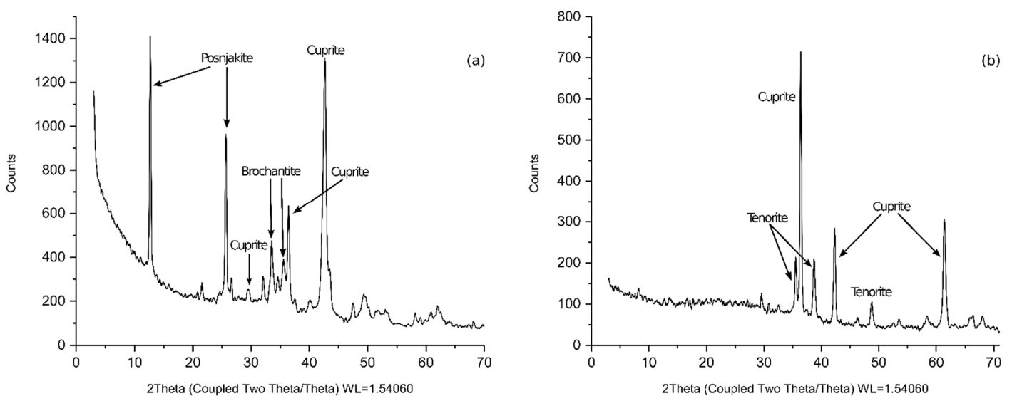
Figure 9. Diffraction patterns of samples E2 (a) and ESP1 (b).
