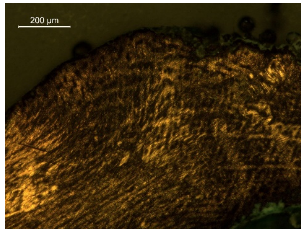
Figure 7. Metallography of the sample showing an as-cast microstructure.
