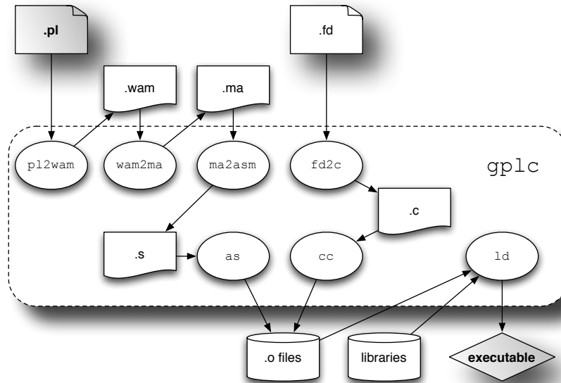
Fig. 1. Compilation Scheme
