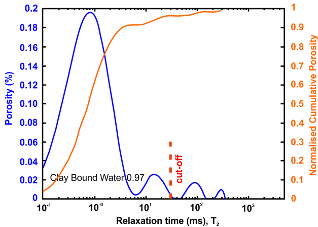
Figure 9. Porosity and cumulative porosity values for sample EPT-2-3 (Eptachori formation) from current study, time-cut off at 30 ms.
