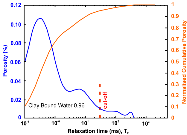
Figure 6. Porosity and cumulative porosity values for sample PENT-3-1 (Pentalofos formation) from current study, time-cut off at 30 ms.
