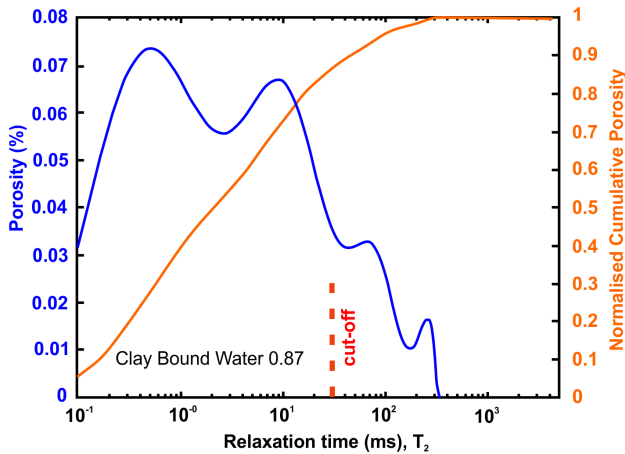
Figure 5. Porosity and cumulative porosity values for sample TSOT-1-3 (Tsotyli formation) from current study, time-cut off at 30 ms.
