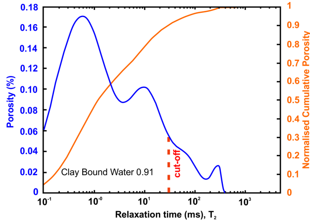
Figure 7. Porosity and cumulative porosity values for sample PENT-3-2 (Pentalofos formation) from current study, time-cut off at 30 ms.
