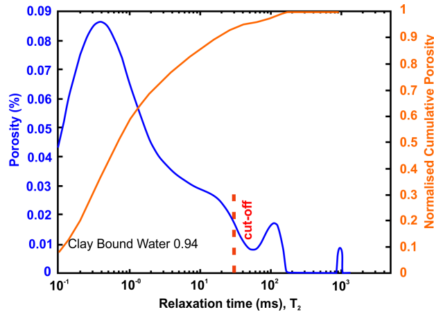
Figure 8. Porosity and cumulative porosity values for sample PENT-3-3 (Pentalofos formation) from current study, time-cut off at 30 ms.
