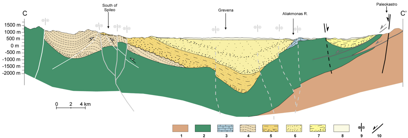
Figure 2. Cross-section from Krania in the West to Paleokastro in the East (cross-section reproduced with permission from Vamvaka, 2010), where 1: Pelagonian nappe, 2: Ophiolites, 3: Jurassic limestones, 4,5,6,7: Krania, Eptachori, Pentalofos, Tsotyli Fms, 8: Quaternary Deps, 9, 10: Strike-slip and dip-slip faults, respectively.
