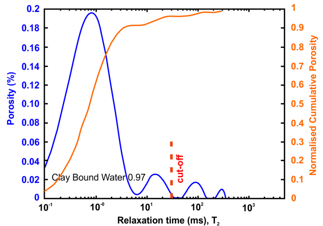
Figure 4. Example of a nuclear magnetic resonance (NMR) result and interpretation. The area under the curve is the total porosity (in %). A standard cut-off value at 30 ms defines the amount of water located in clays. This cut-off can however vary depending on the value of surface relaxivity r_2 (i.e. the type of clays).
