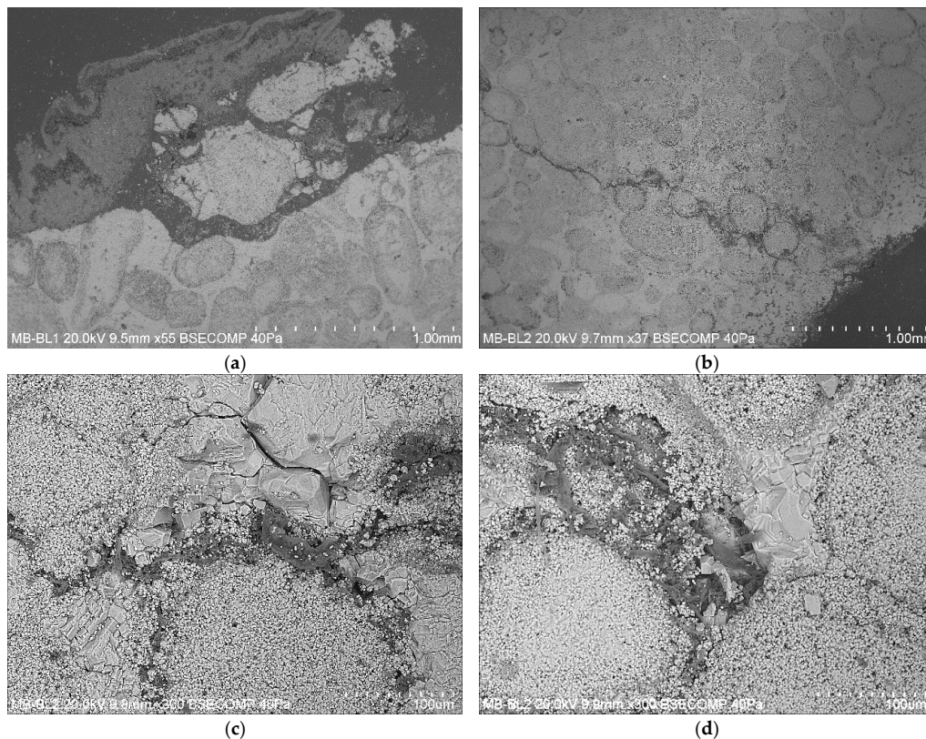
Figure 5. Back-scattered imaging detector (BSEM) micrographs of biodeteriorated Batalha oolitic limestone: (a) Detached stone fragments incorporated within the growing lichenous weathering crust; (b–d) Lichen hyphae penetrating deeply inside the limestone fabric using pre-existing intracrystalline cracks and/or porosity within the sparitic cement and leading to the detachment of the oolitic grains.
