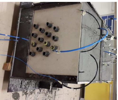
Figure 6.1.5. Module side and top construction. OPC + EPS insulating concrete appearance. b) Scaling up of thermal performance of the minimodule
