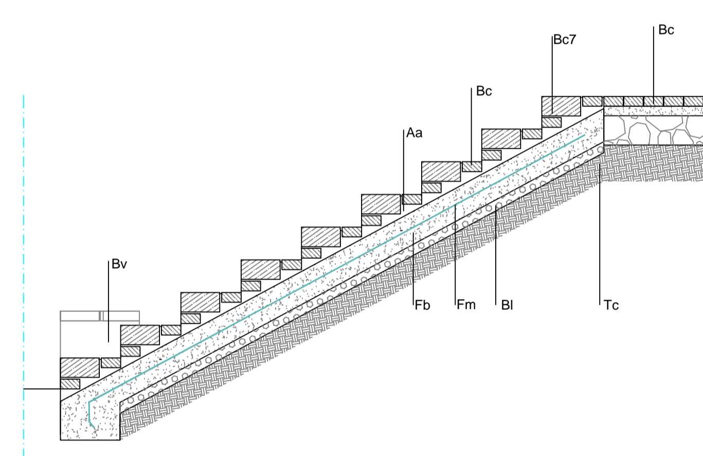
Pormenor 6 - Esc: 1/20
