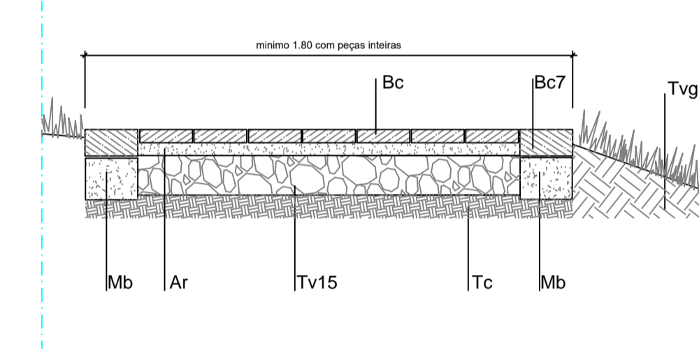
Pormenor 7 - Esc: 1/20
