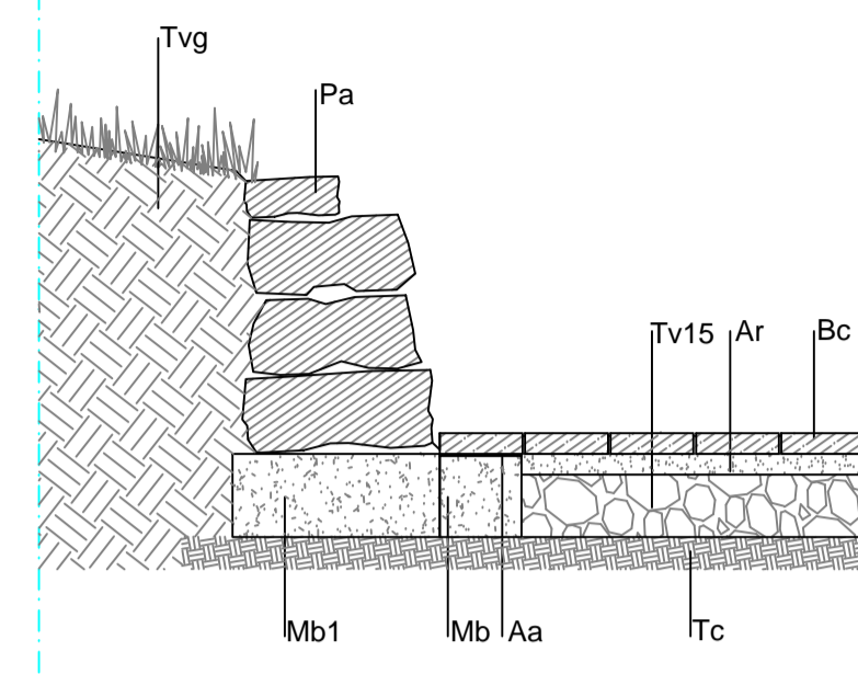
Pormenor 1 - Esc:1/20
