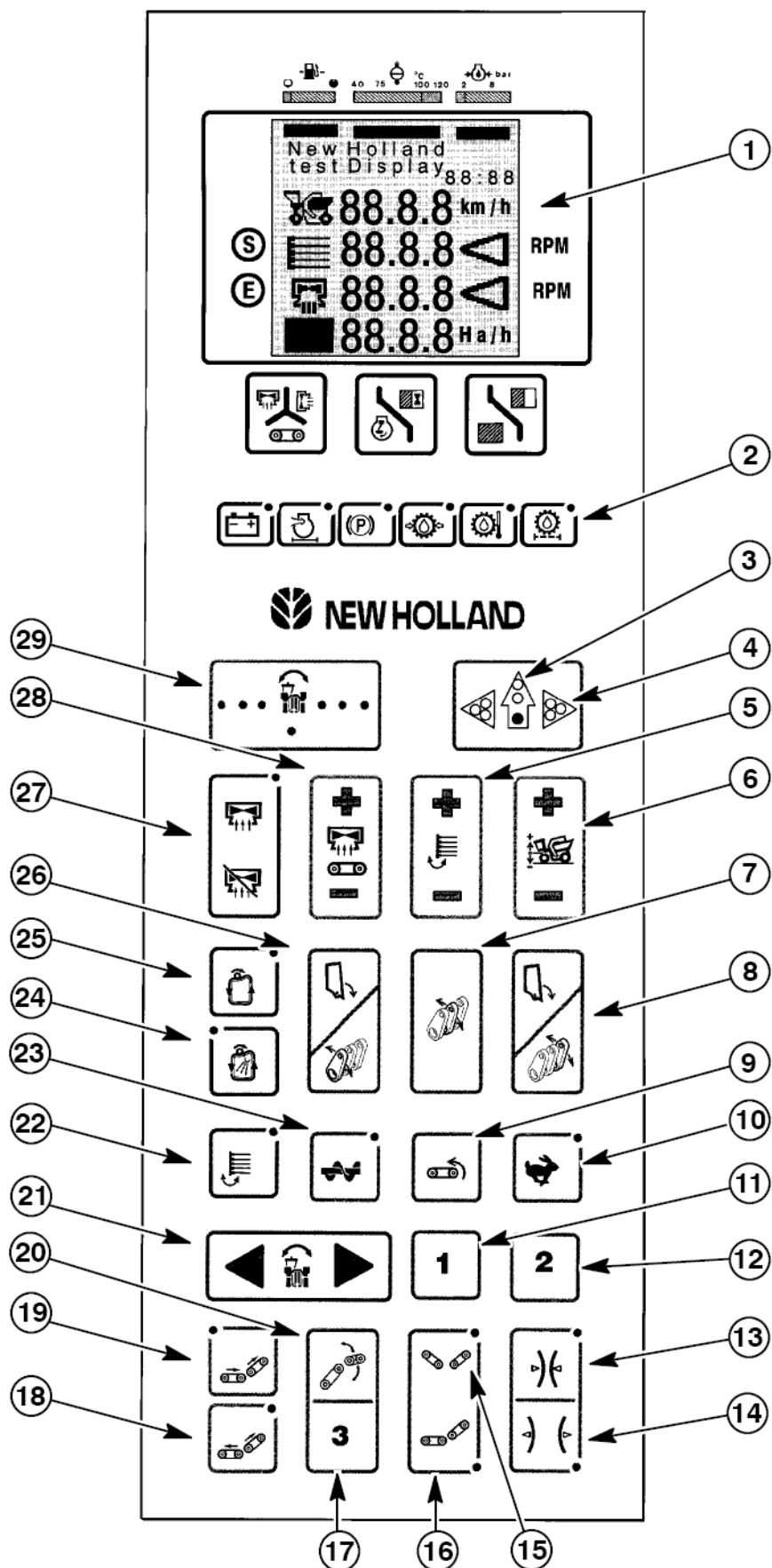
Fig. 1.39 http://www.newholland.com
