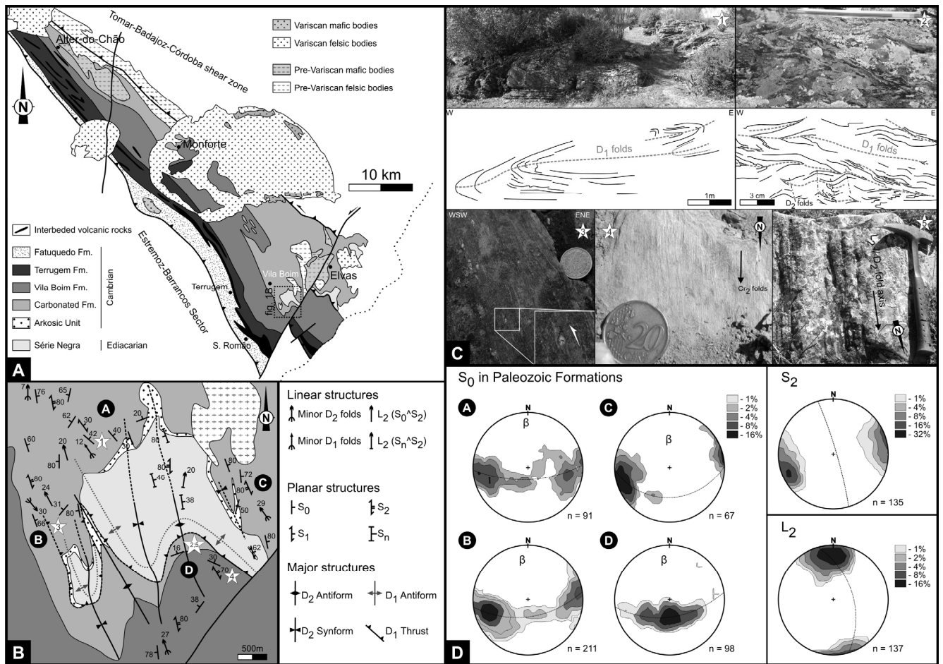
Fig. 1. A. Geological sketch from Alter-do-Chão-Elvas Sector, with reference to the Torre de Cabedal structure location (adapted from Carvalho et al. , 1992); B. Geological and structural map of Torre de Cabedal structure (geological limits partially adapted from Gonçalves & Assunção, 1970); C. Structures observed in study area: 1 and 2 - D 1 recumbent folds in Carbonated Fm., 3 - D 1 thrust criteria, top to SW, 4 - D 2 crenulation cleavage in pelites from Vila Boim Fm., 5 - D 2 open folds in Fm. Carbonated (location in Fig 1B); D. Point diagram density relating to poles of bedding planes (S 0 ) for four sections of the structure, second deformation event cleavage (S 2 ) and intersection lineations (L 2 ) – Schmidt lower hemisphere.
